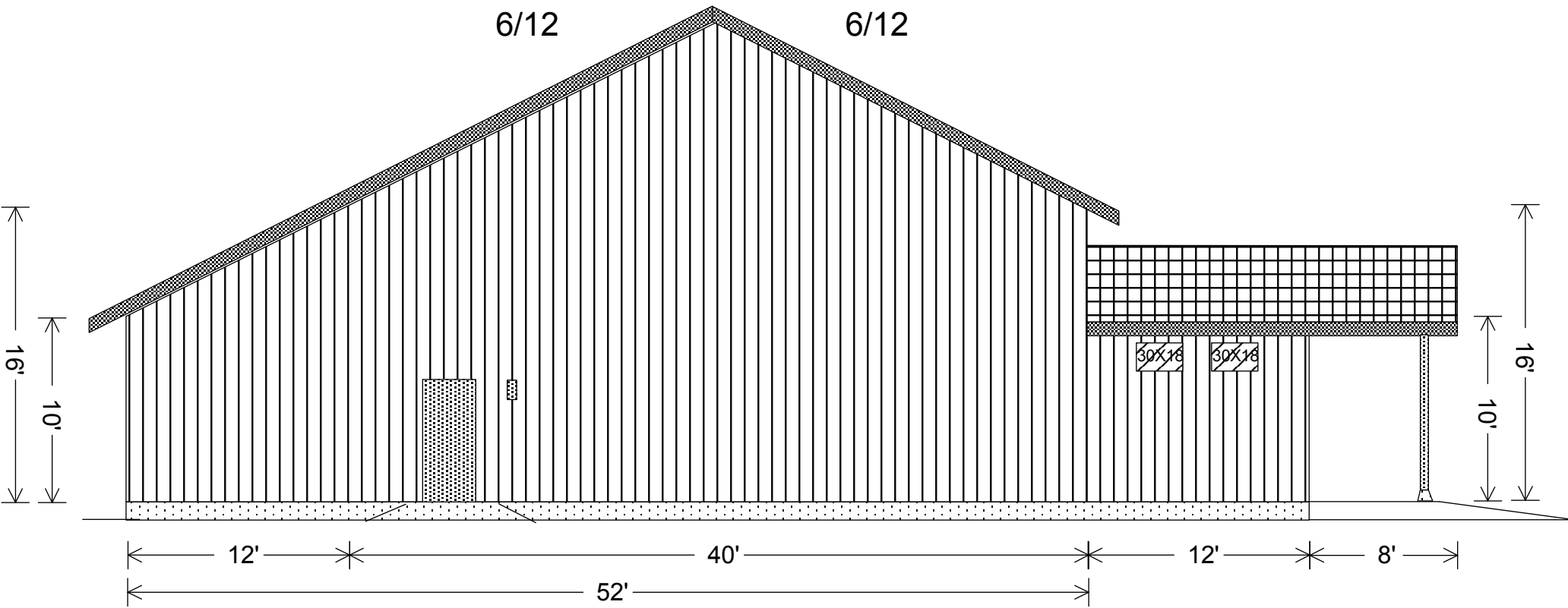
SOUTH ELEVATION 4-2-24
